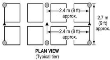
(1) Single Row Racks
