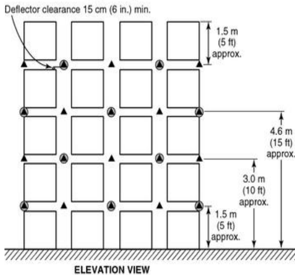
▲ Flue sprinkler ● Face sprinkler Note: Face sprinklers must be staggered vertically; line up in-rack sprinklers with transverse flue spaces. (2) Double Row Racks up to 7.6 m (25 ft) High Storage
