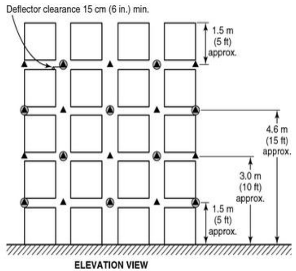
▲ Flue sprinkler ● Face sprinkler Note: Line up in-rack sprinklers with transverse flue spaces; face sprinklers must be staggered vertically. (3) Multiple Row Racks up to 7.6 m (25 ft) High Storage
