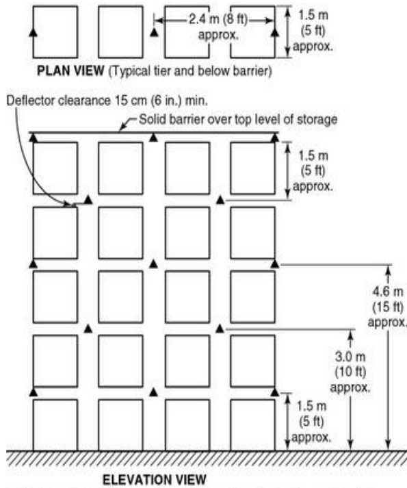
(1) Single Row Racks
