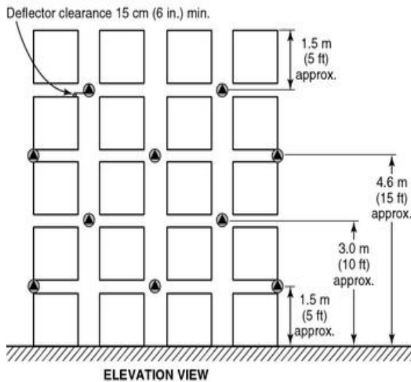
(2) Double Row Racks
