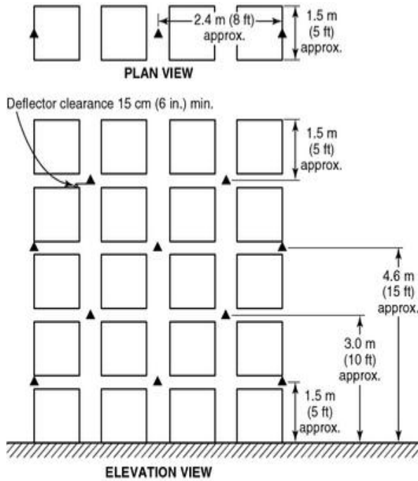
(1) Single Row Racks
