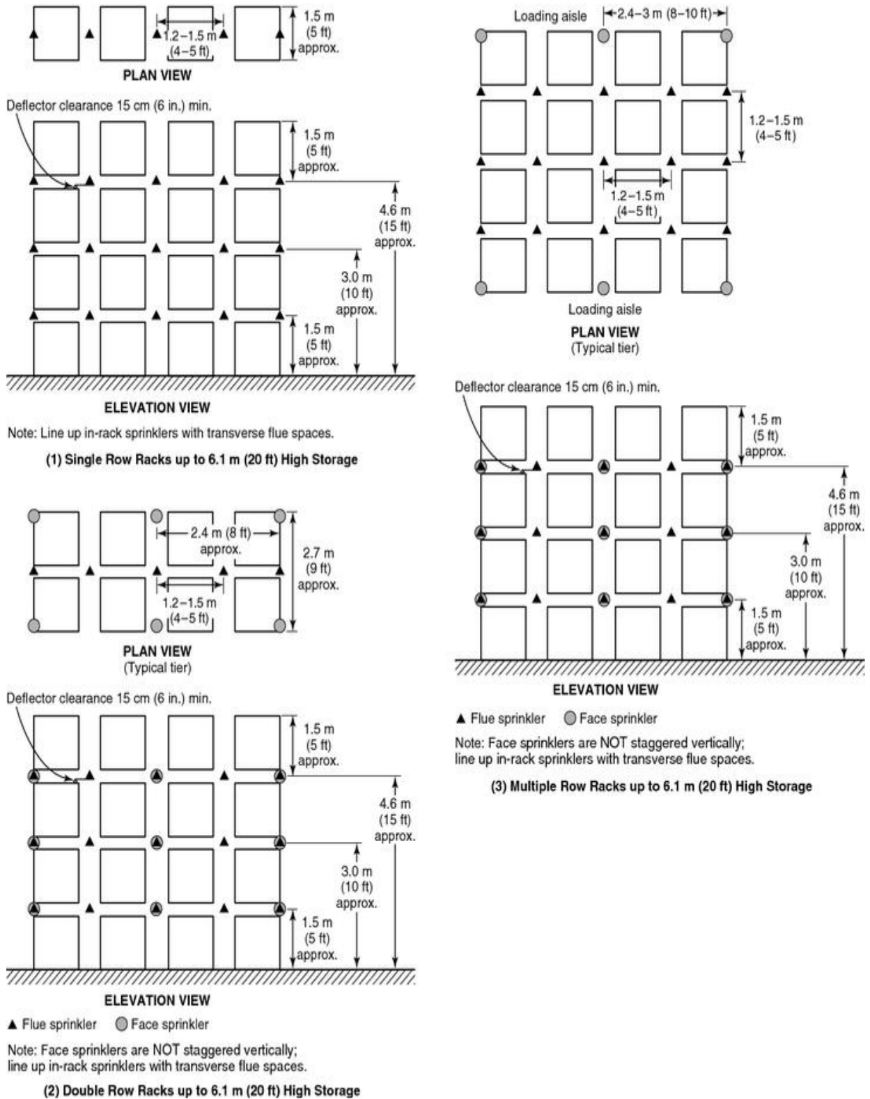
FIGURE 6.3.2.7(d) In-Rack Sprinkler Layout, Uncartoned Level 2 and Level 3
