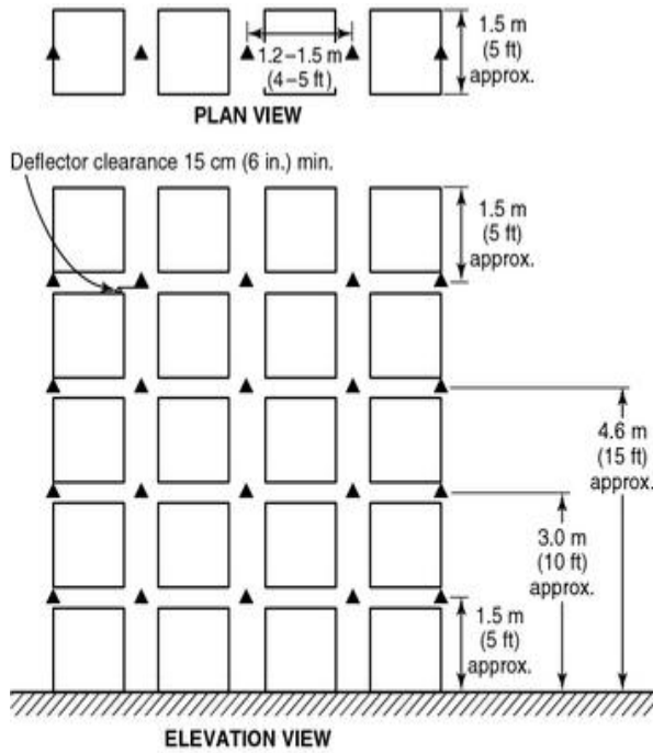
Note: Line up in-rack sprinklers with transverse flue spaces. (1) Single Row Racks up to 7.6 m (25 ft) High Storage
