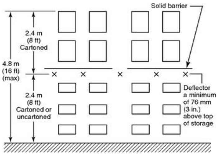
ELEVATION VIEW
